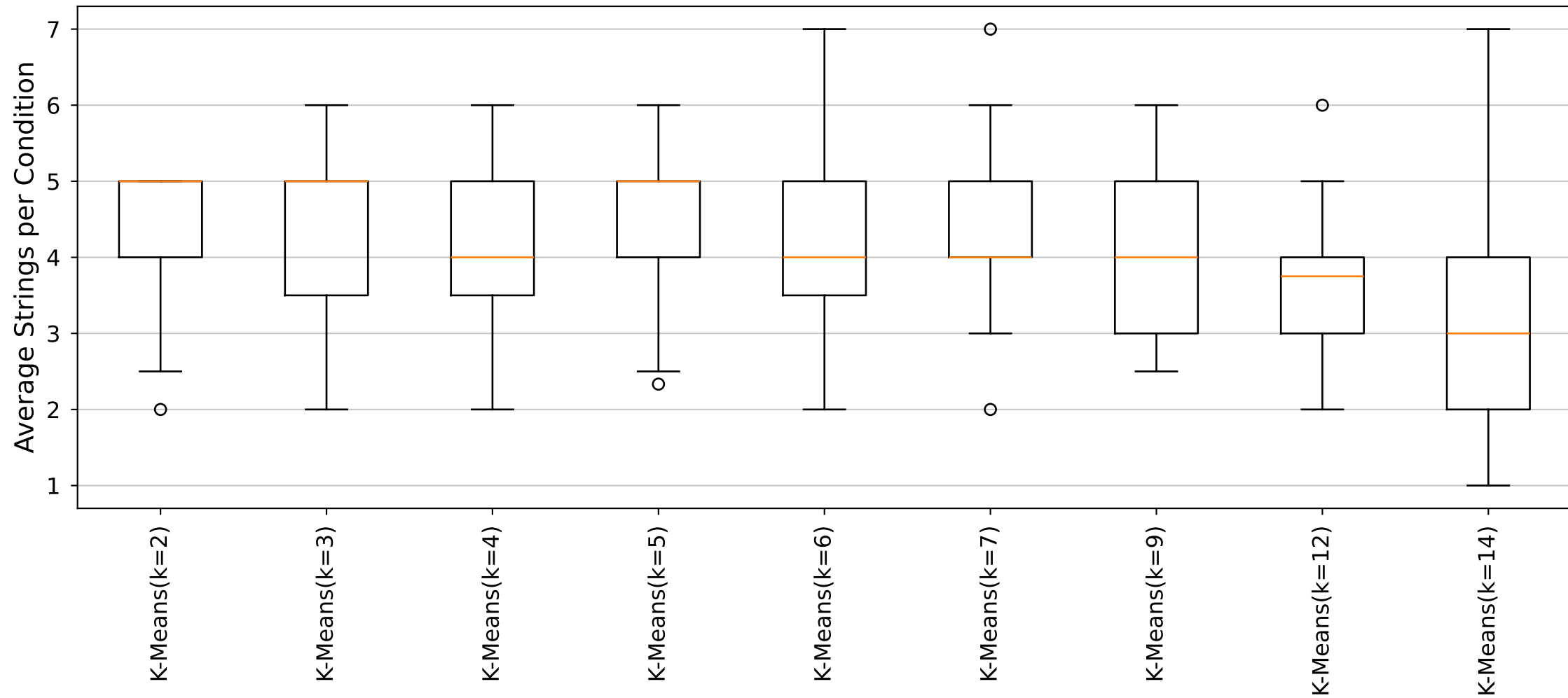
YARA Rules Average Strings per Condition Distribution (Cluster7_Size14 dataset)
